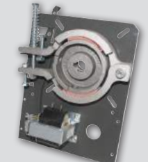
Brake Assembly For PRO-J/H 120 Volt Solenoid Included MX00037-120V
